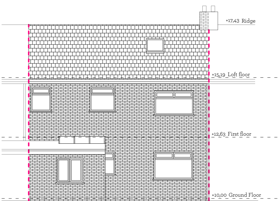
Garden Elevation
