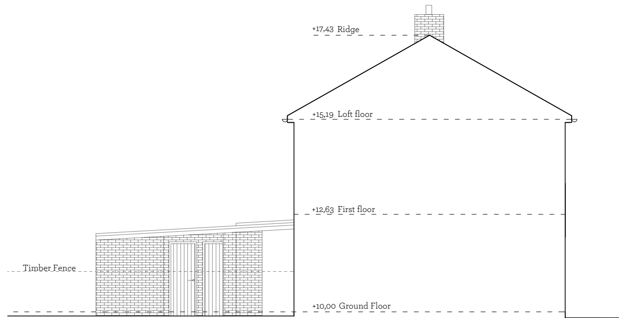
Side Elevation View from property No. 45
