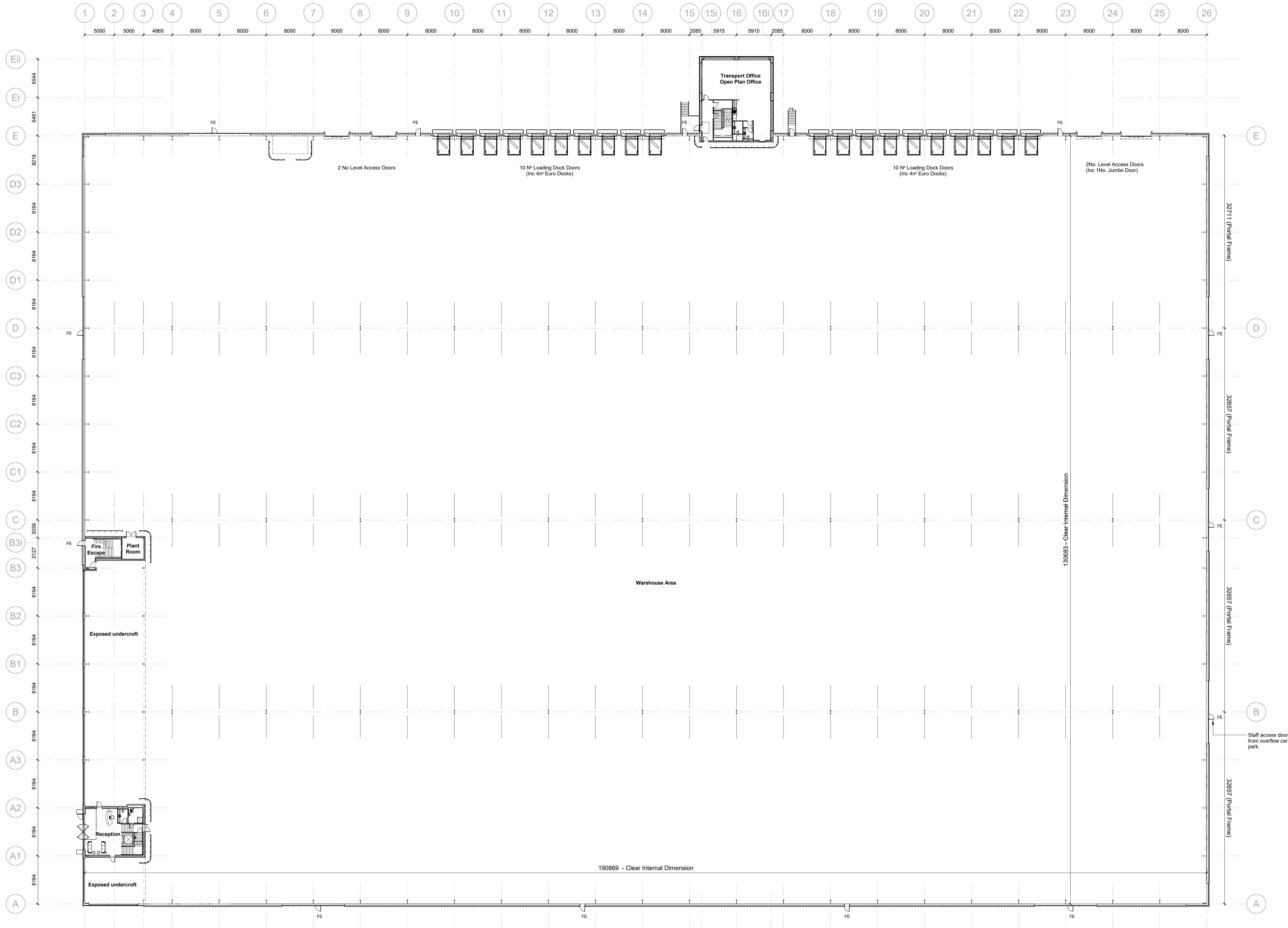
Unit 03 - Building Plan 1 : 250
