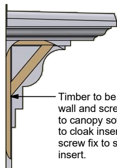
Auxiliary View Showing Bracket Fixing ( 1:20 )
