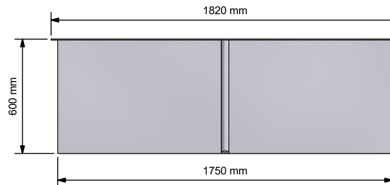
Plan View ( 1:20 )
