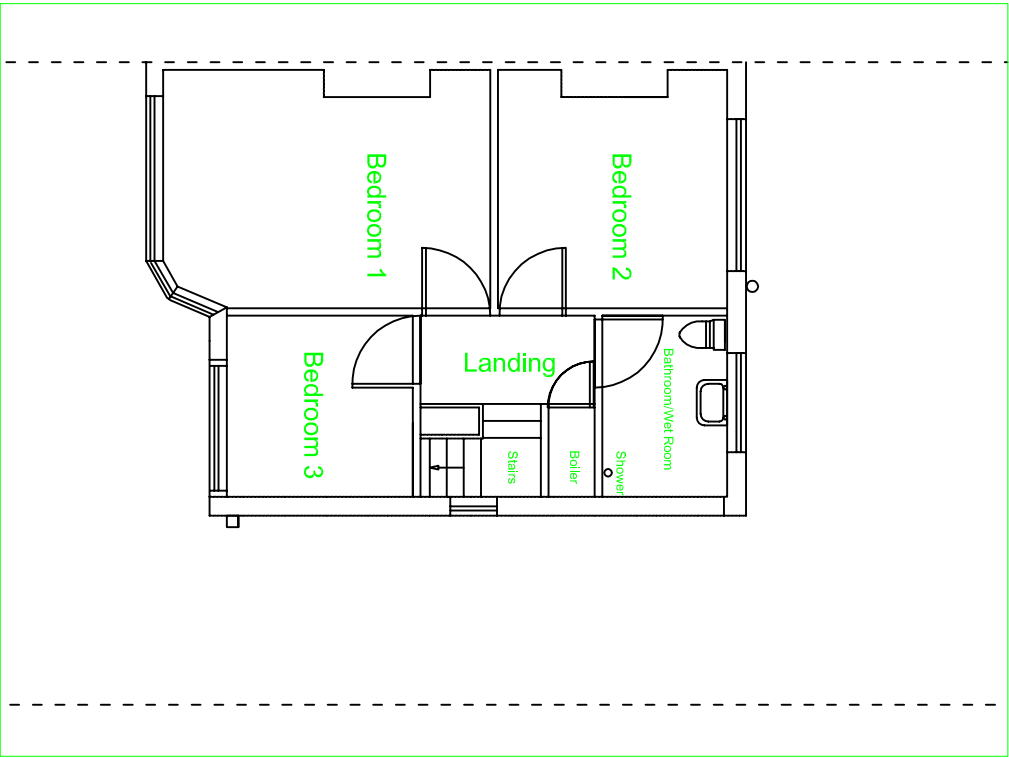
Existing First Floor Layout
