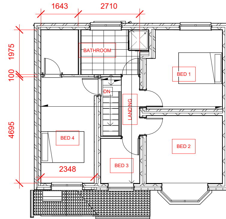
2 Level 1ST 1 : 100
