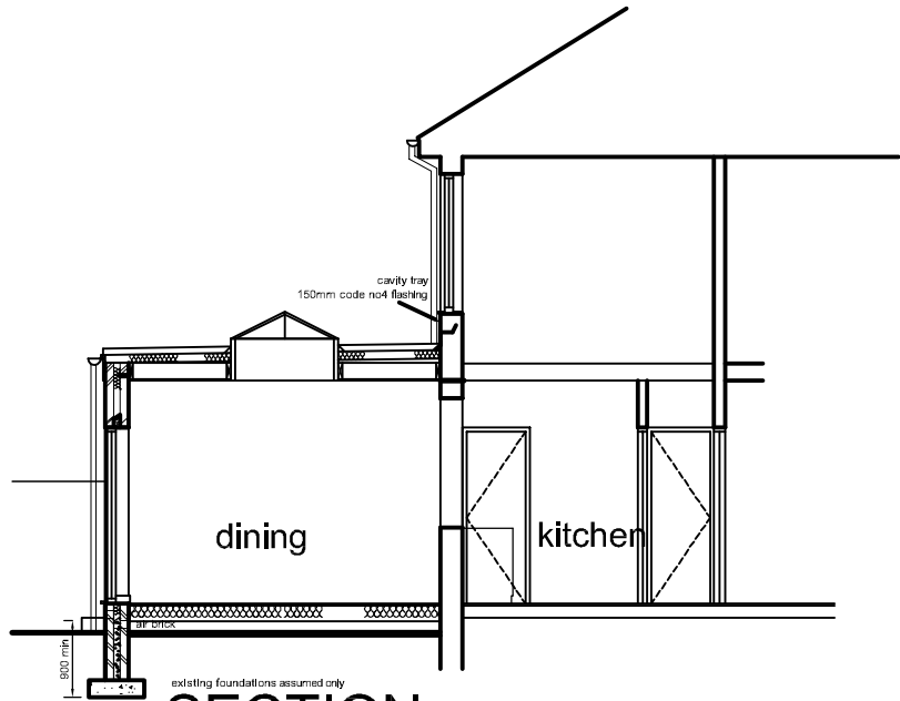
SECTION
