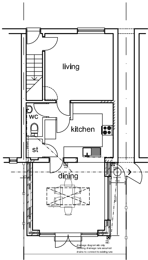
GROUND PROPOSED
