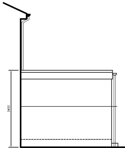
SIDE
