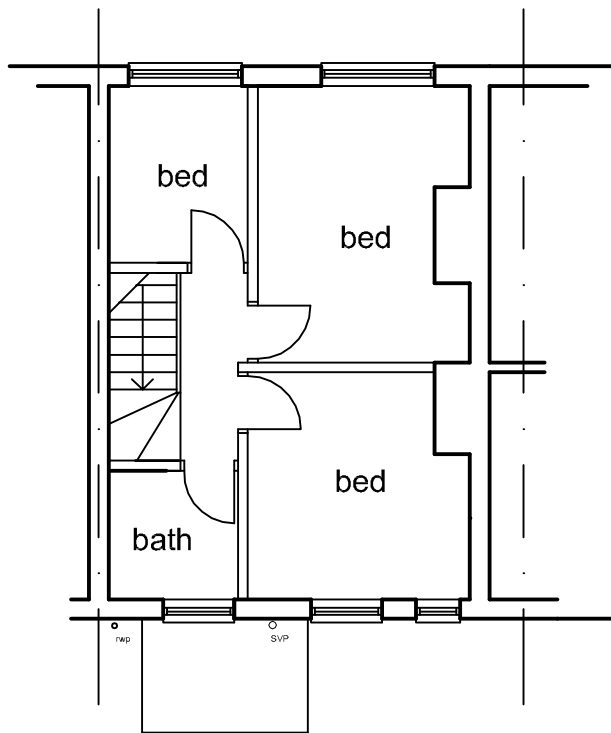
FIRST EXISTING
