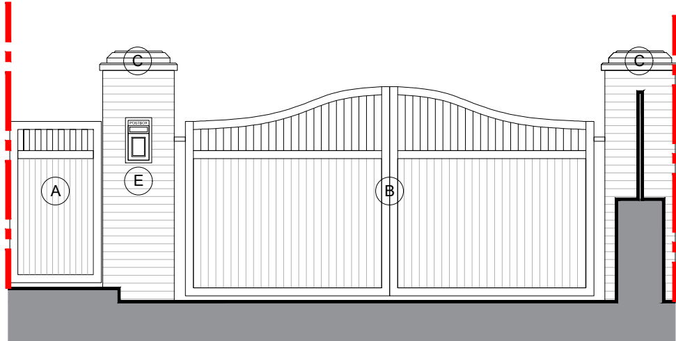
Proposed Front Gate Elevation @ 1:50
