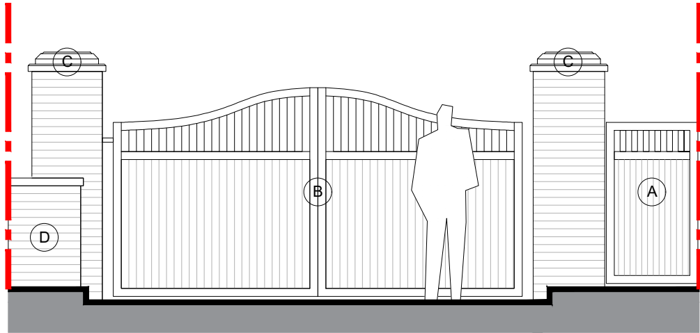
Proposed Rear Gate Elevation @ 1:50
