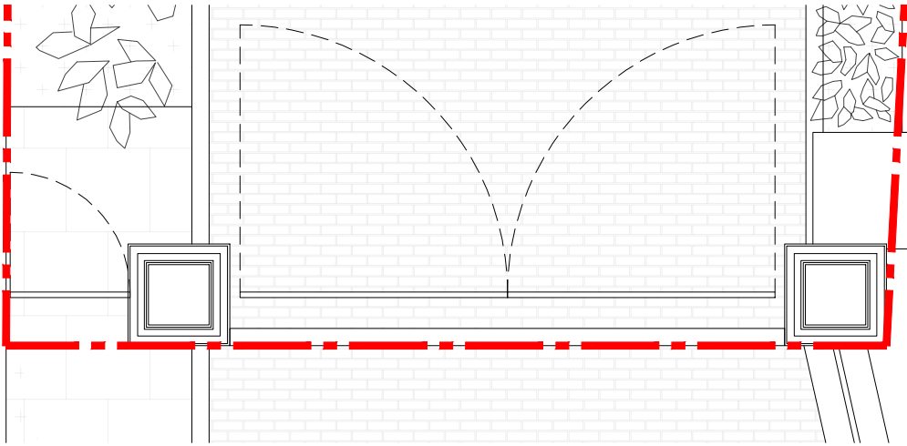
Existing Front Gate Plan @ 1:50
