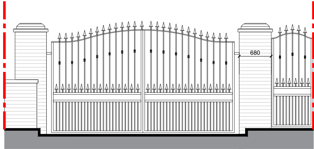
Existing Rear Gate Elevation @ 1:50
