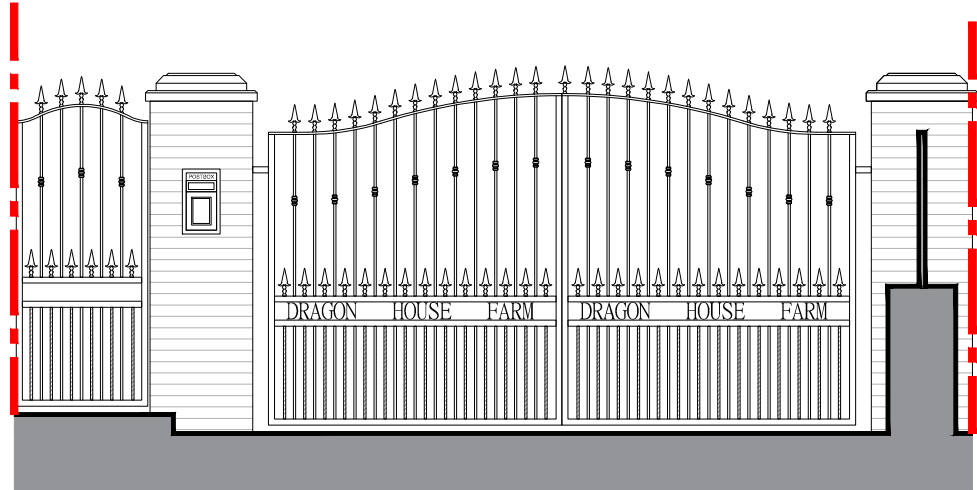
Existing Front Gate Elevation @ 1:50
