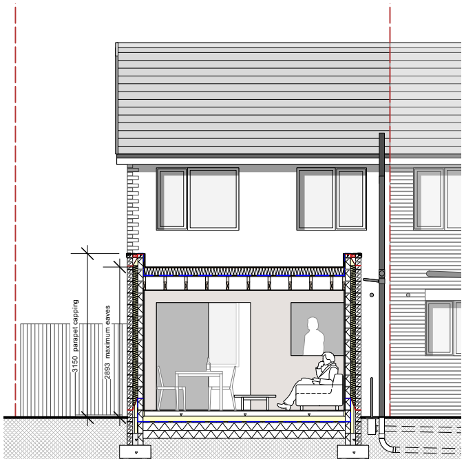
Eaves and Parapet height section
