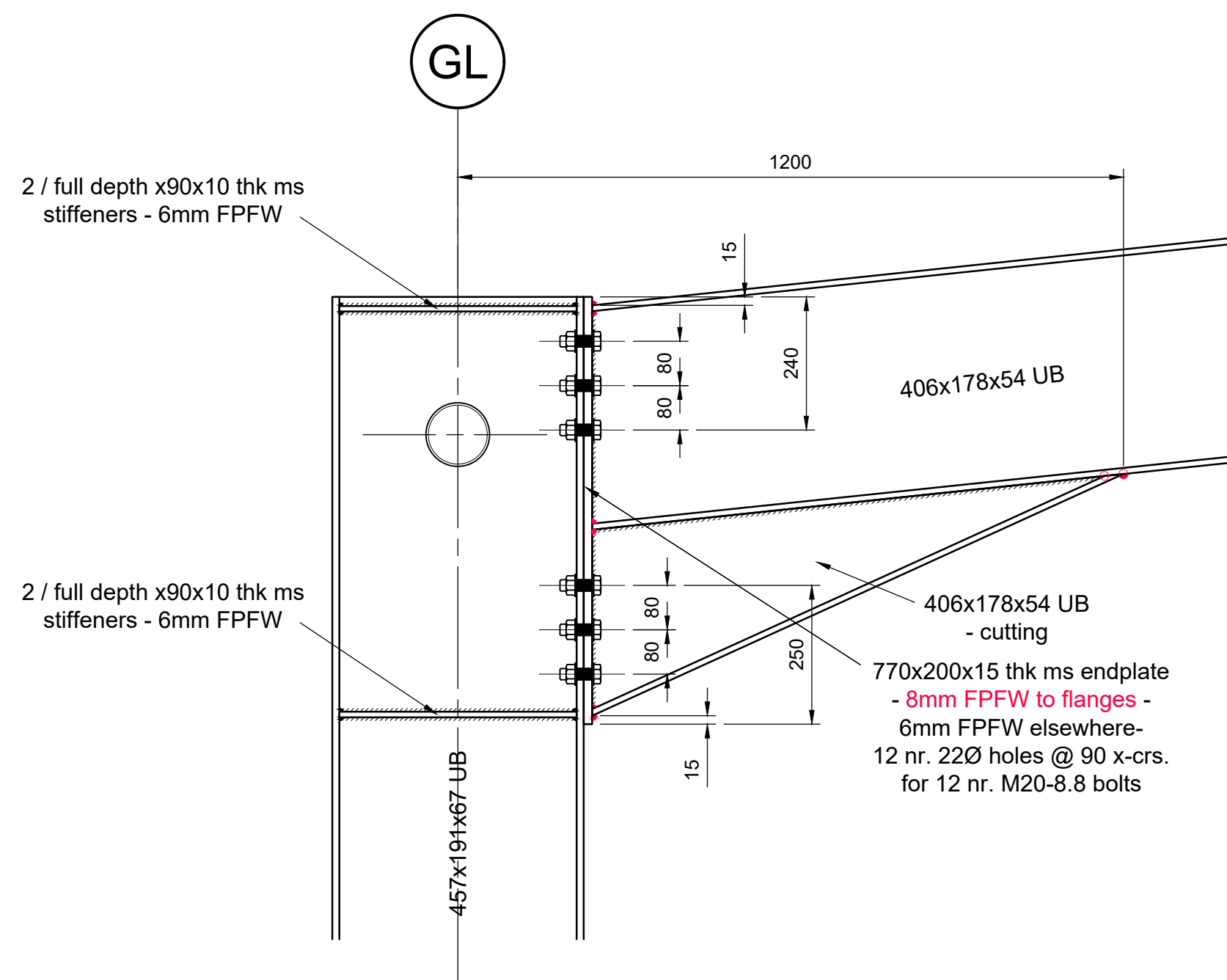
Eaves connection detail
