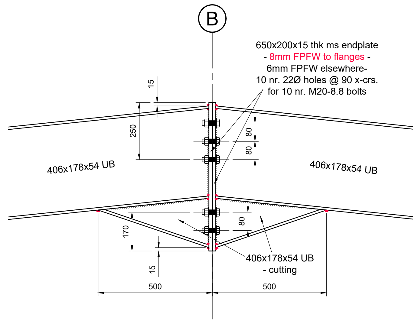
Apex connection detail
