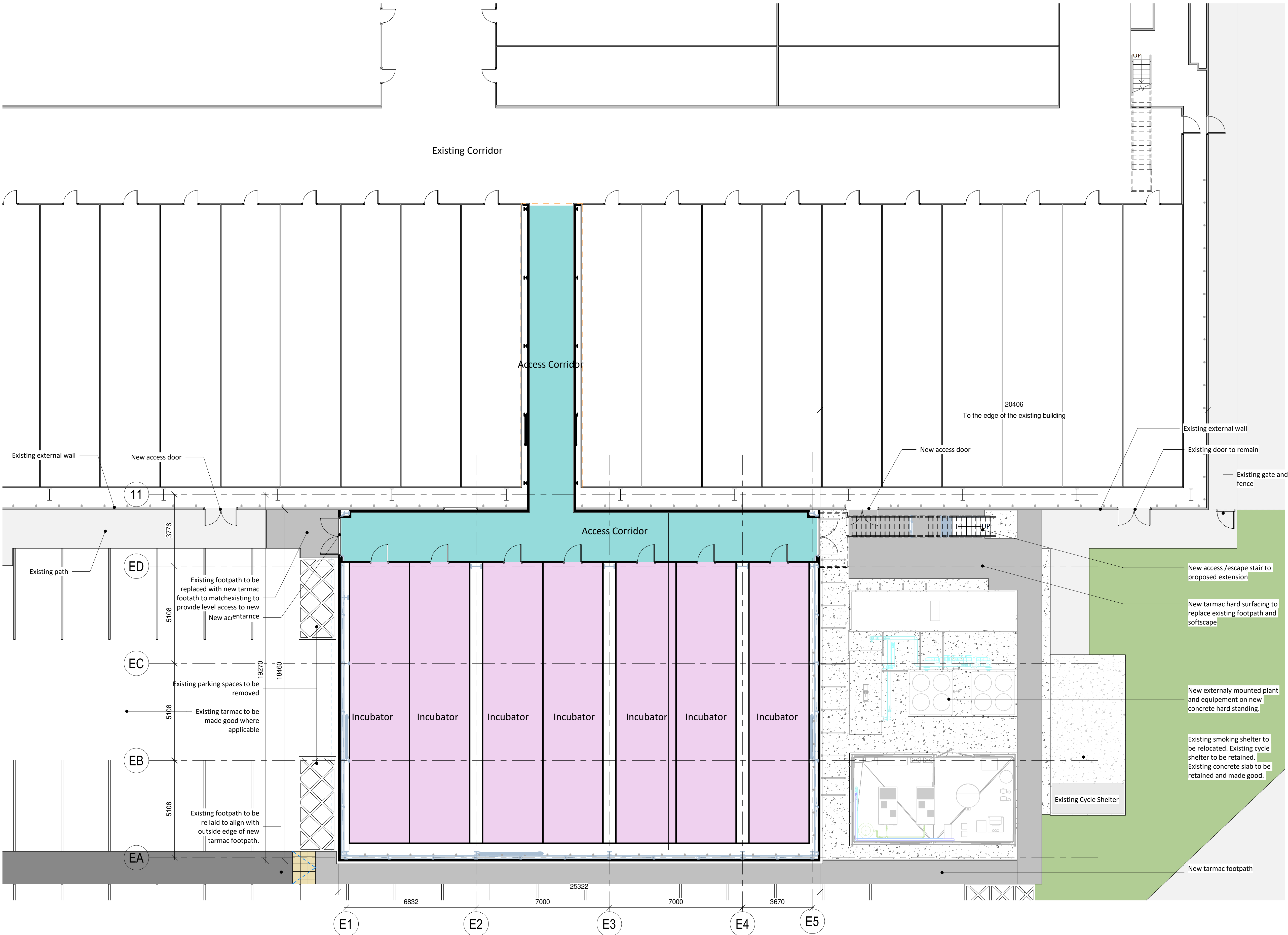
Proposed Ground Floor GA Plan Planning Scale: 1 : 100
