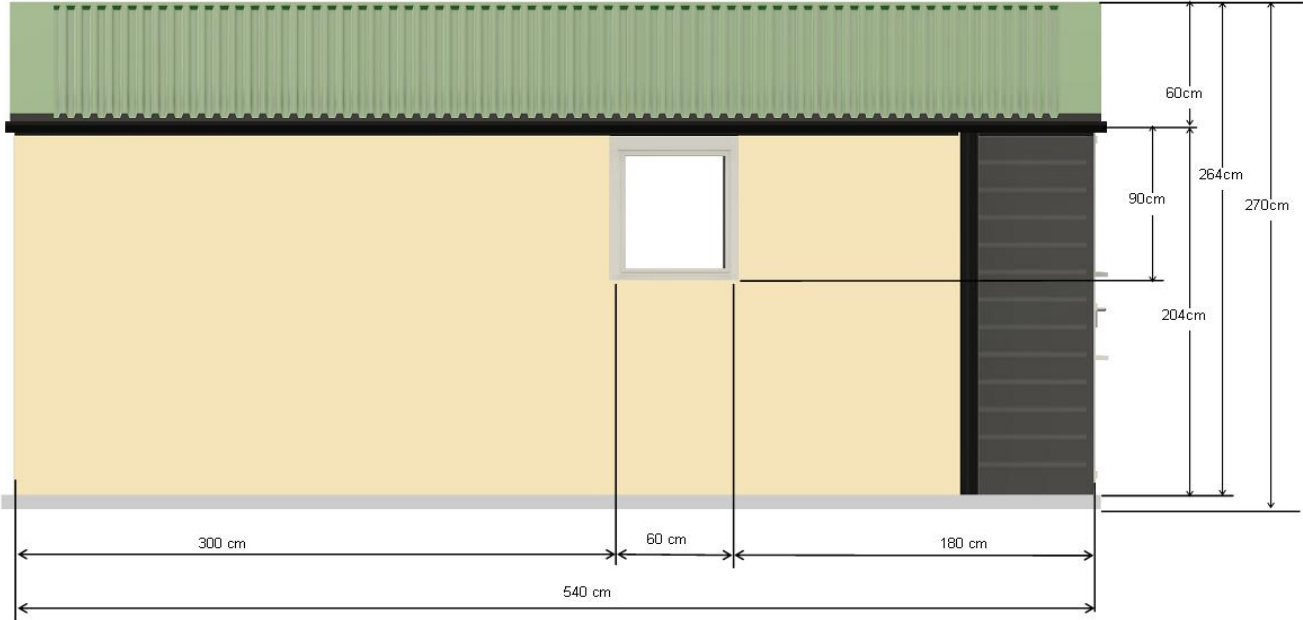
Left Elevation
