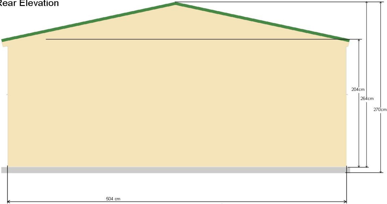
Rear Elevation
