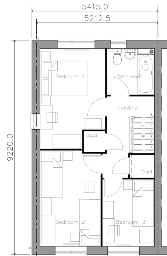
First Floor Plan GFA 41.83m 2 (41.03m 2 )
