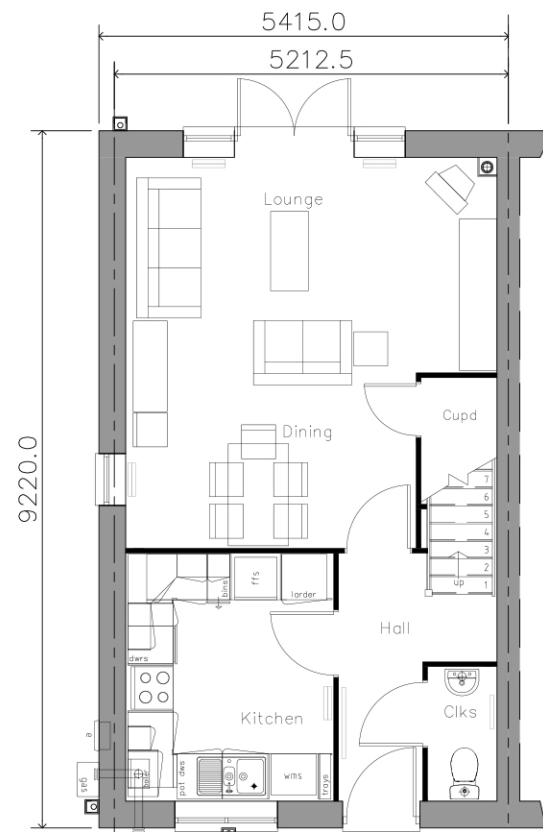
Ground Floor Plan GFA 41.83m 2 (41.03m 2 )
