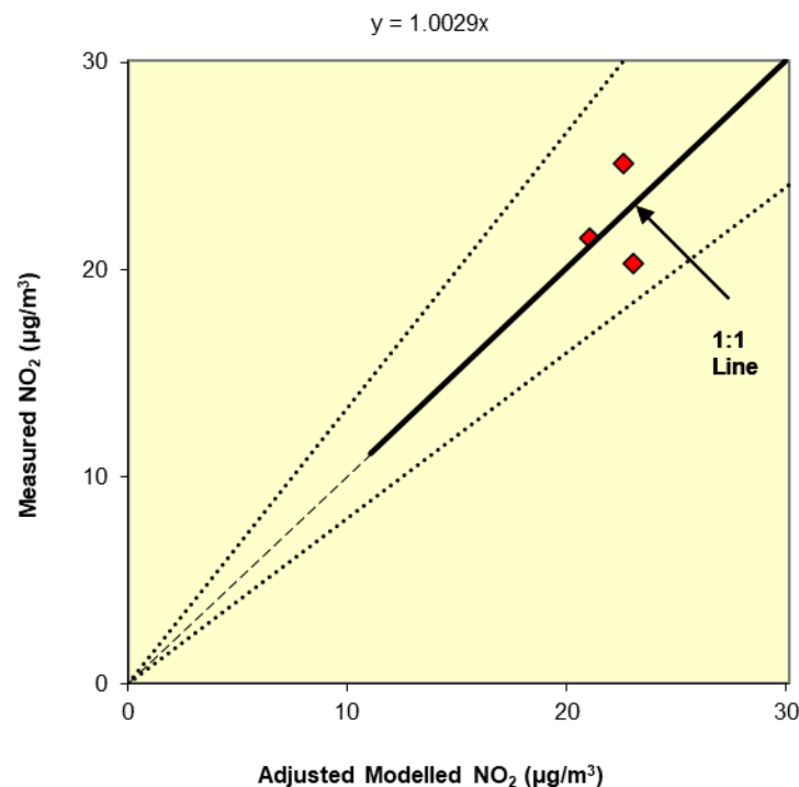
Figure 10.3.3: Comparison of Measured Total \text{NO}_2 to Final Adjusted Modelled Total \text{NO}_2 Concentrations. The dashed lines show \pm 25\% .
