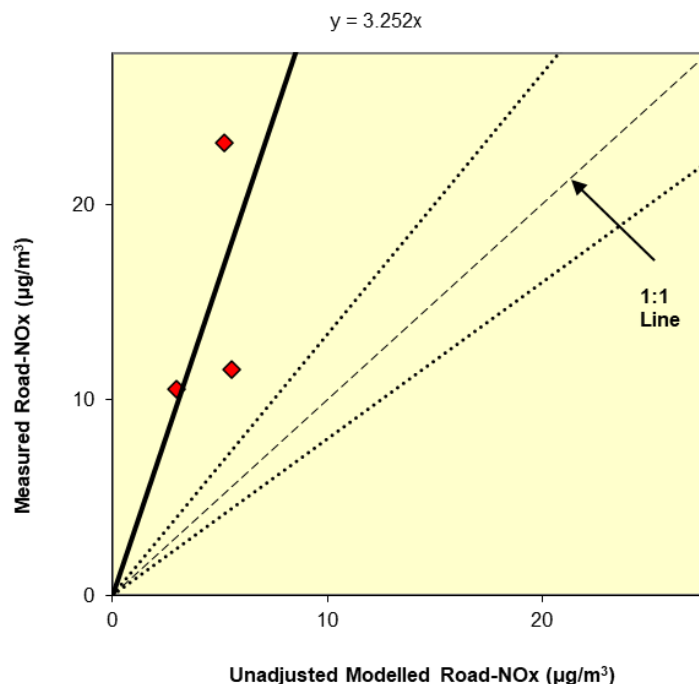
Figure 10.3.2: Comparison of Measured Road \text{NO}_x to Unadjusted Modelled Road \text{NO}_x Concentrations. The dashed lines show \pm 25\% .
