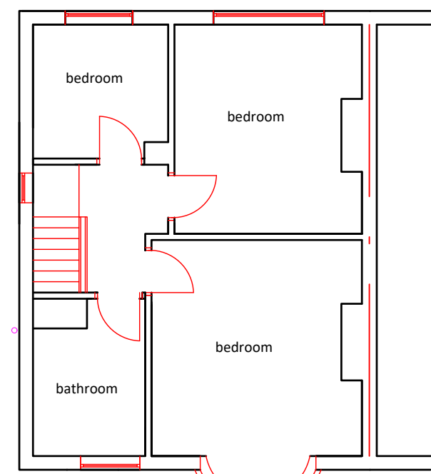
Existing first floor layout
