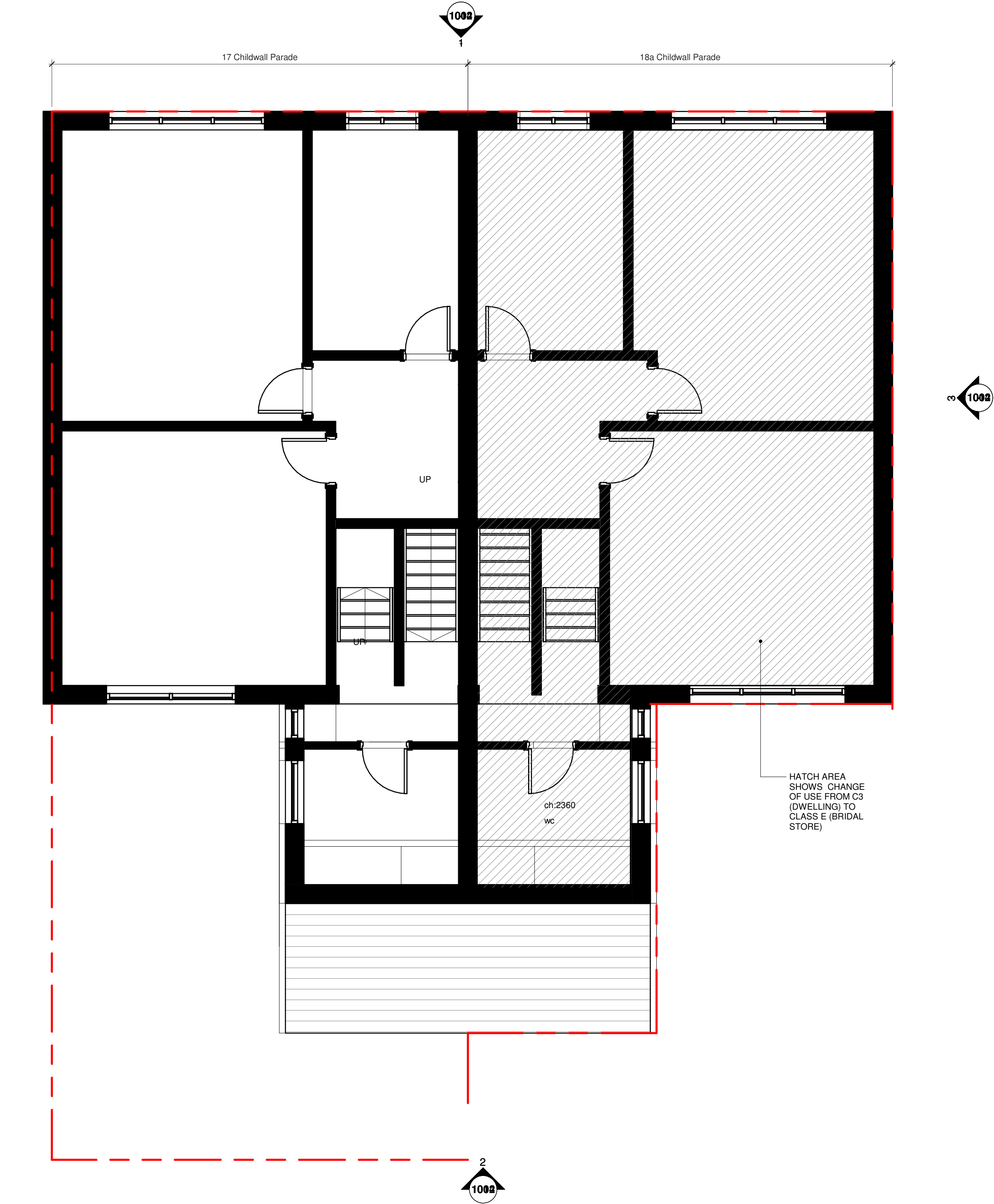
2 Proposed First Floor Scale: 1 : 50
