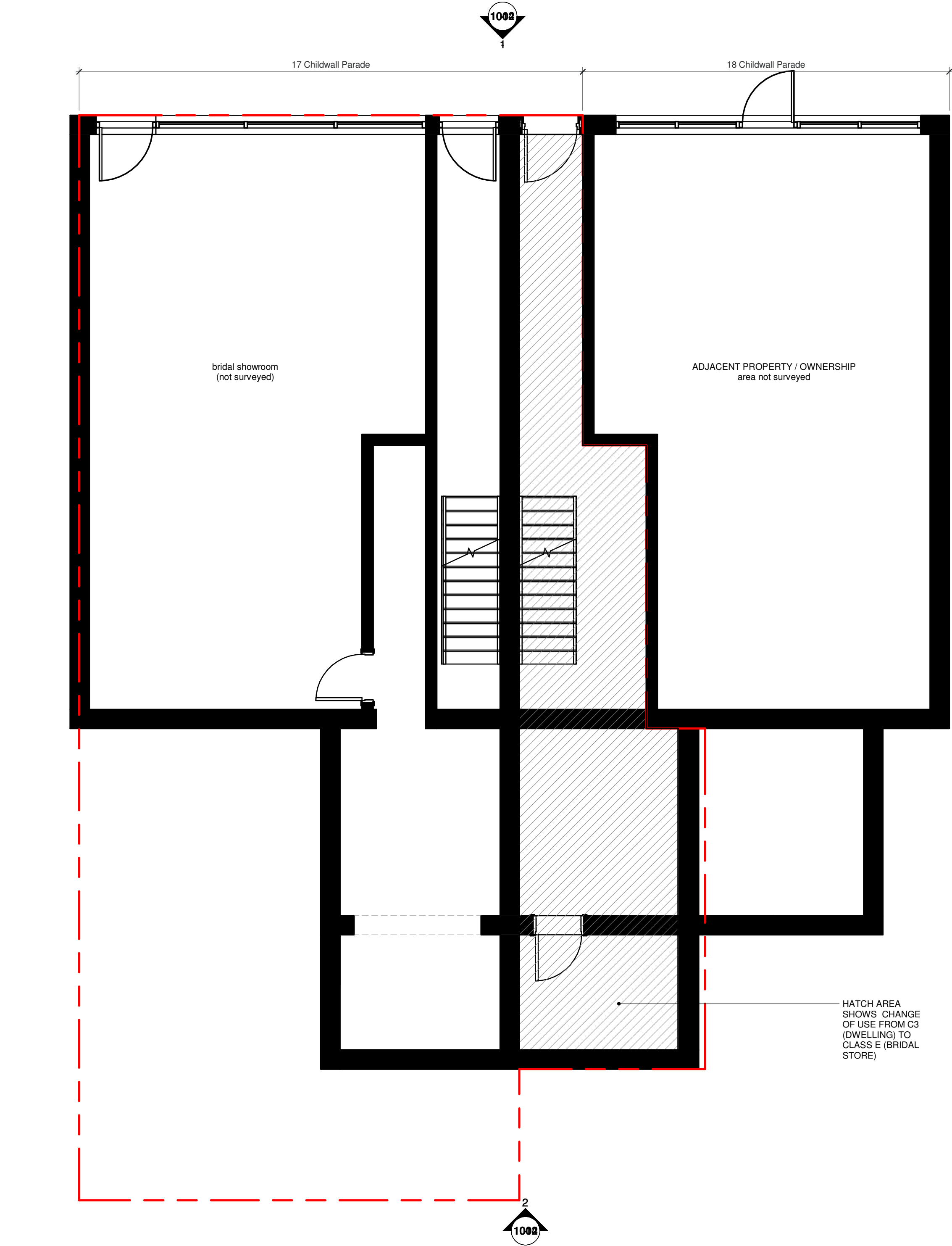
1 Proposed Ground Floor Scale: 1 : 50
