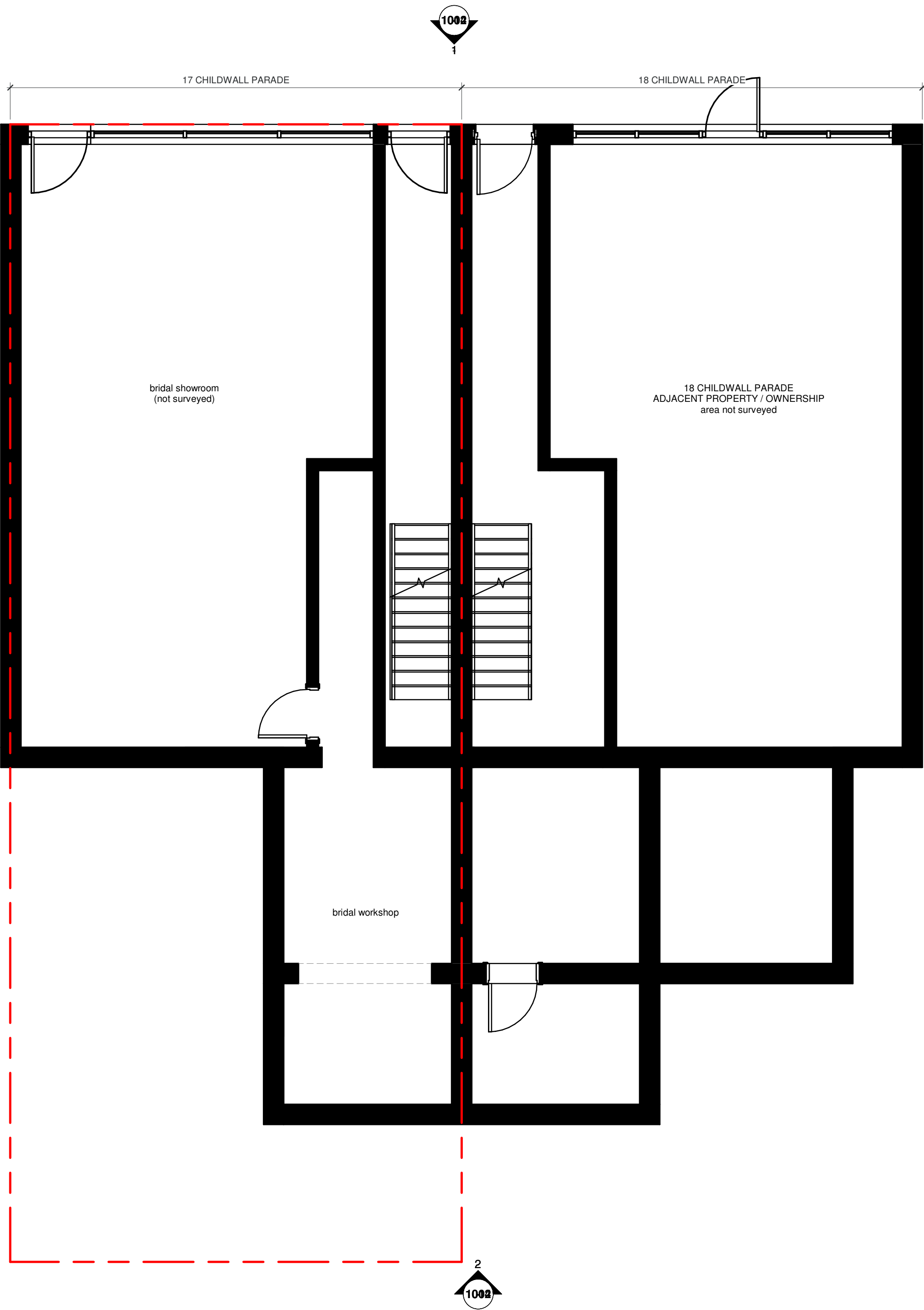
1 Ground Floor Existing Scale: 1 : 50
