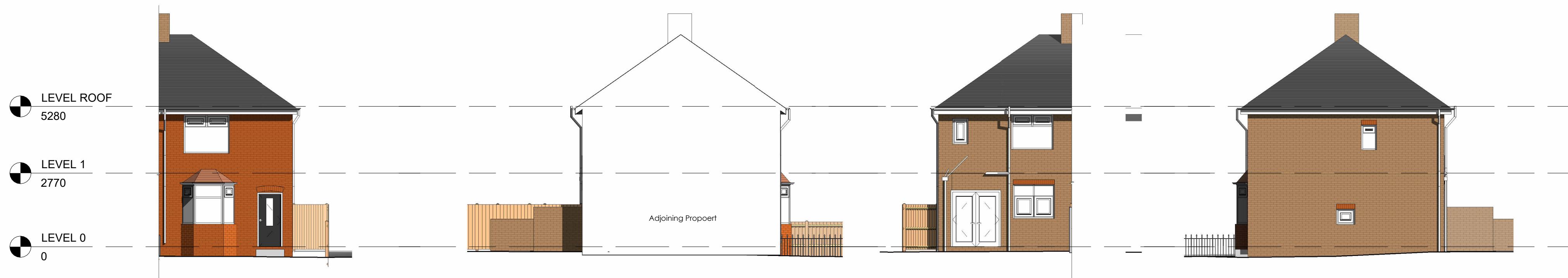
3 Front - Existing 1 : 100
