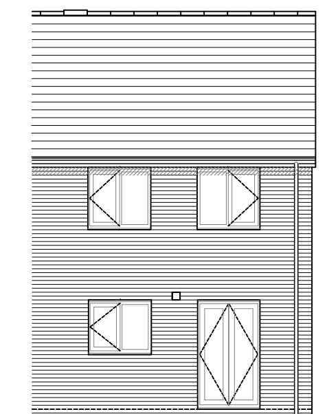
REAR ELEVATION
