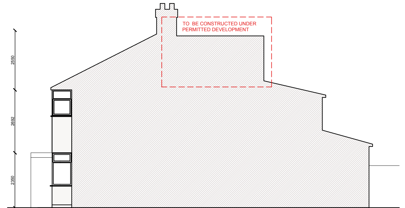
SIDE ELEVATION
