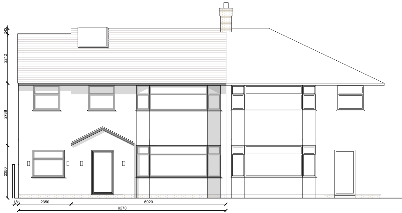
FRONT ELEVATION
