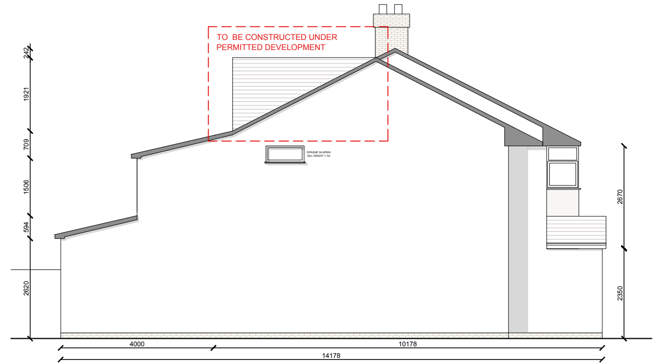
SIDE ELEVATION
