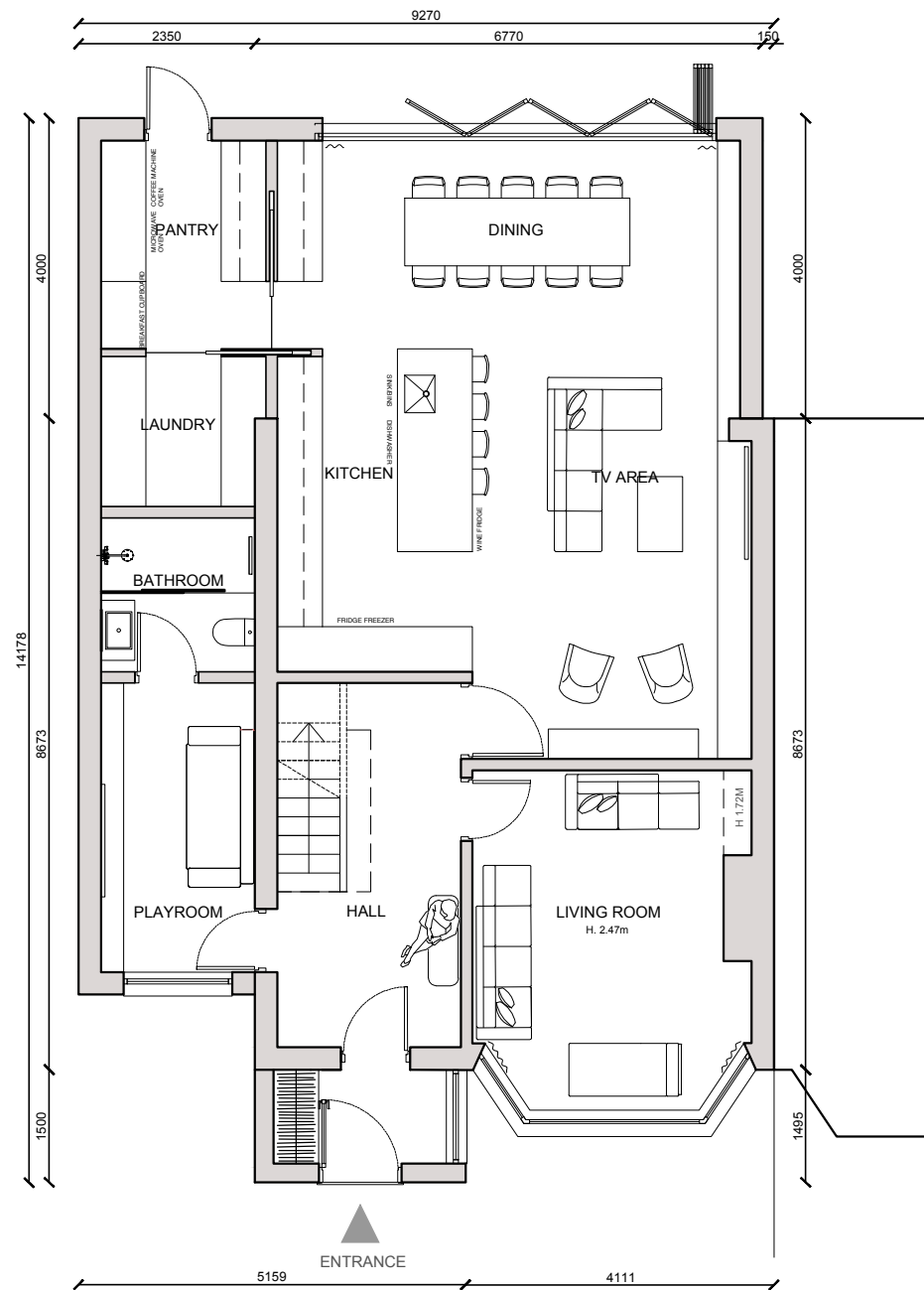
GROUND FLOOR
