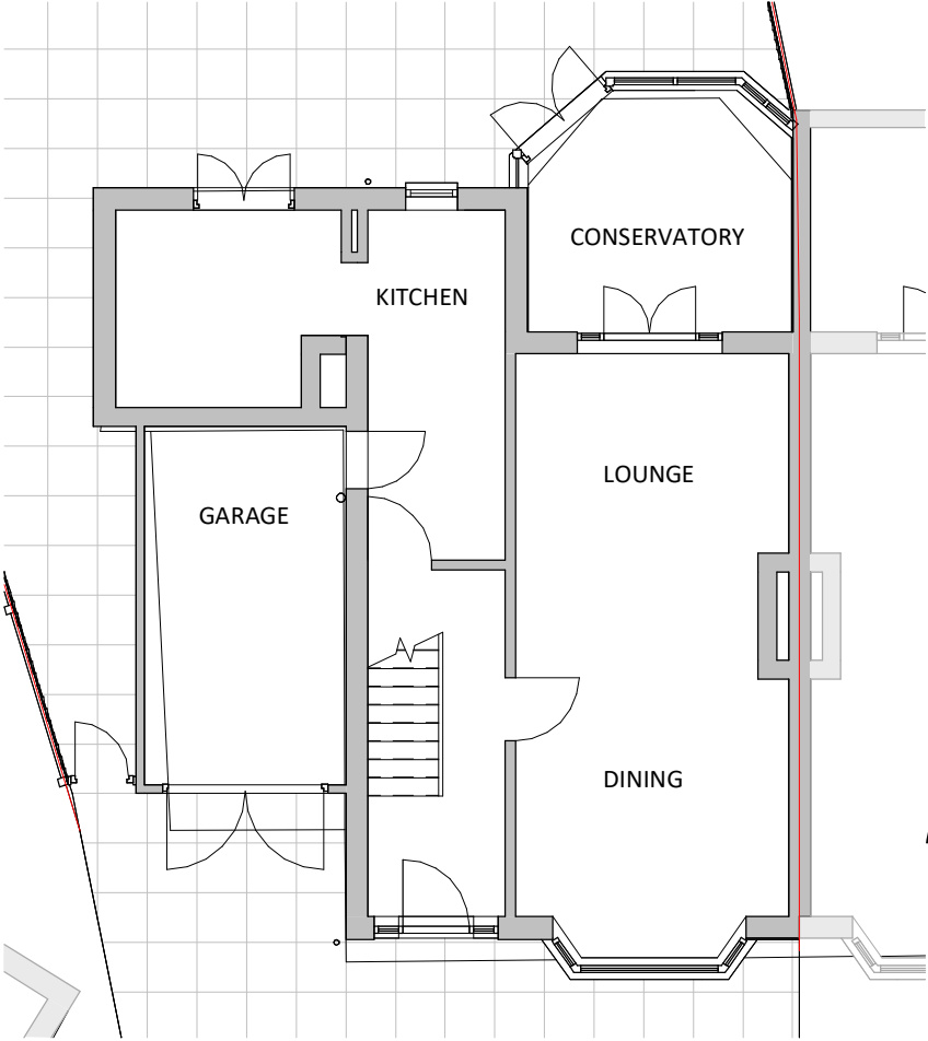
GF PLAN
