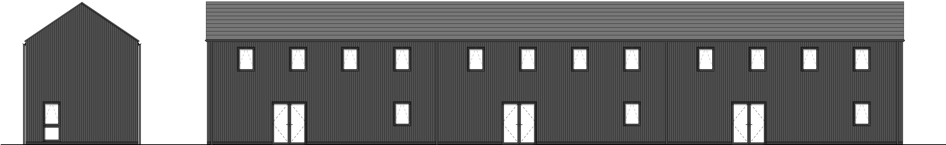
Side Elevation [West]
