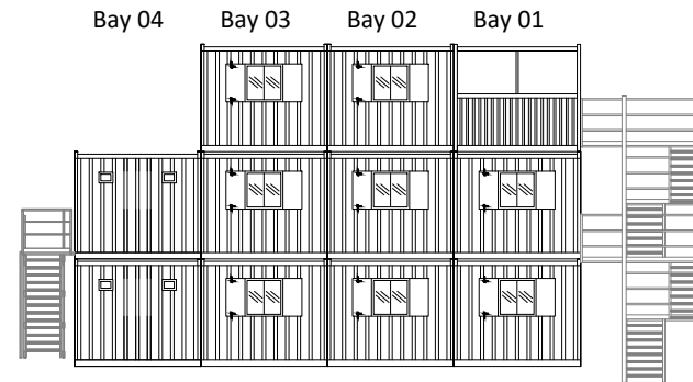
Rear Elevation
