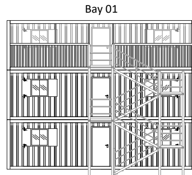
Side Elevation 1
