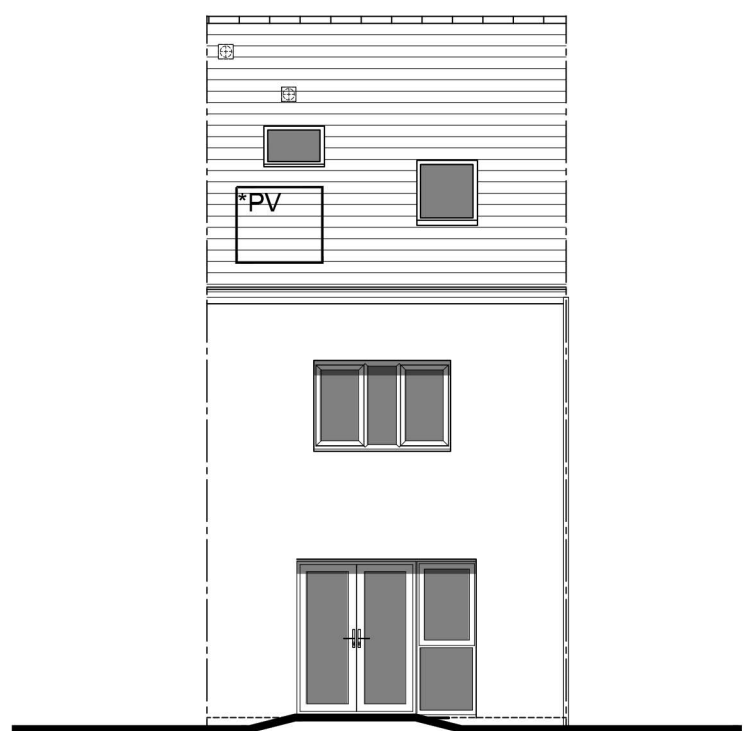
REAR ELEVATION
