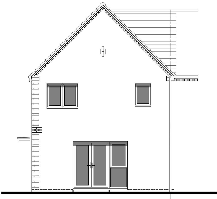
SIDE ELEVATION
