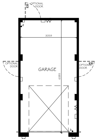
SINGLE GARAGE PLAN
