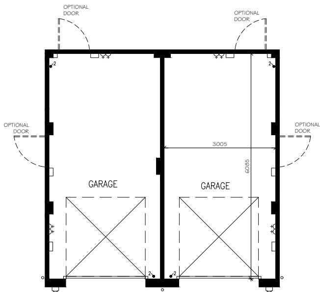
TWIN GARAGE PLAN
