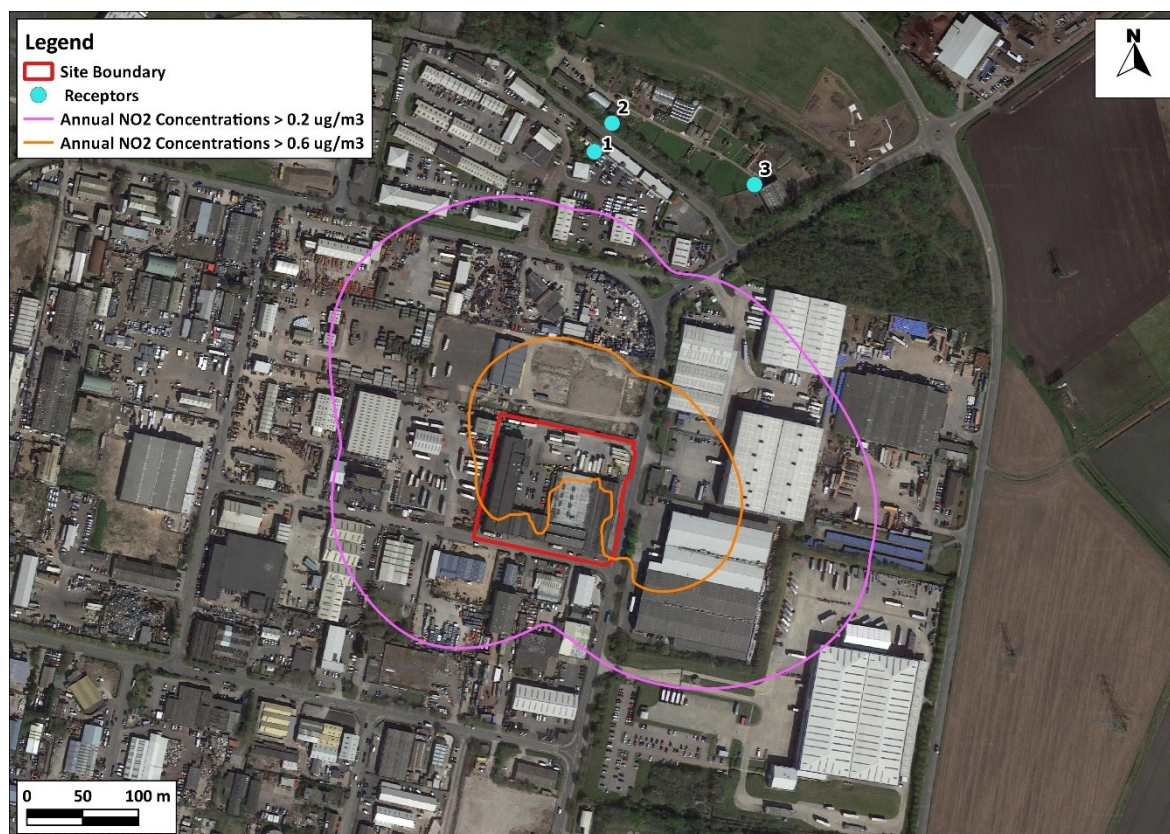
Figure 4: Annual \text{NO}_2 Contours – Proposed Plant Only
