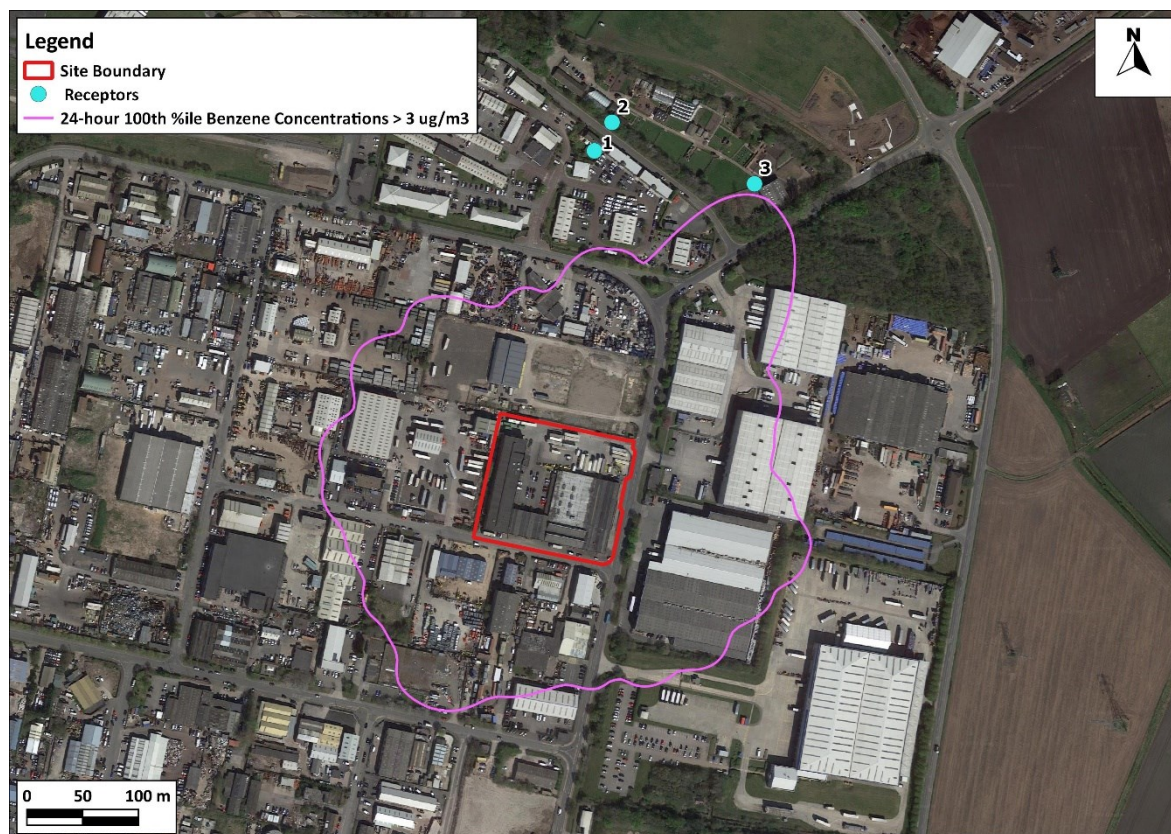
Figure 5: Short-Term Benzene Contour – Proposed Plant Only
