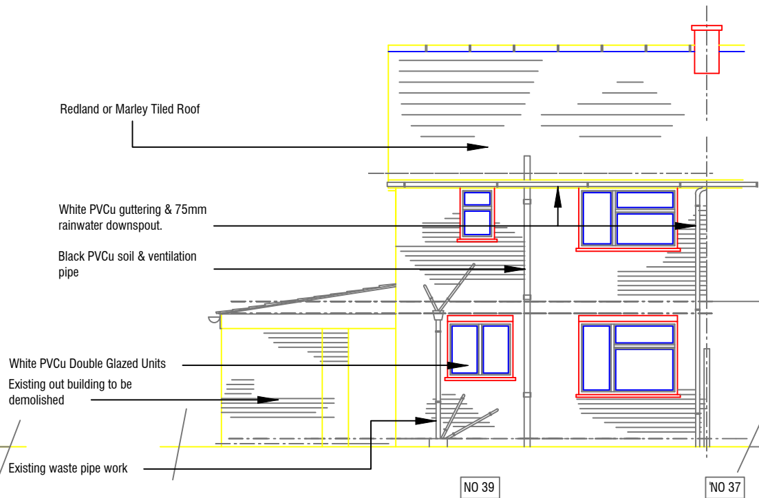
Rear Elevation - As Existing
