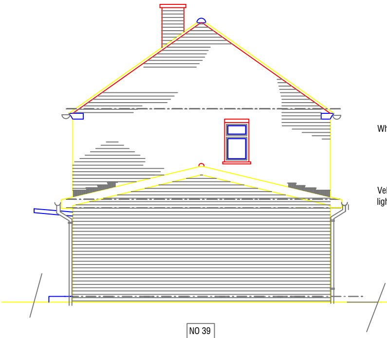
Gable Elevation - As Proposed
