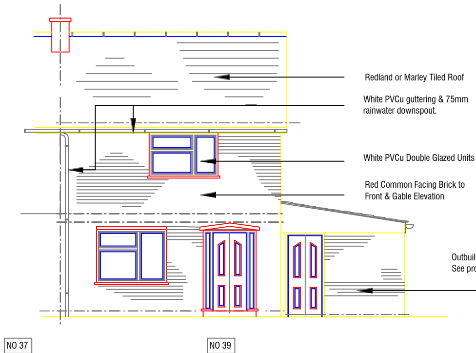
Front Elevation - As Existing
