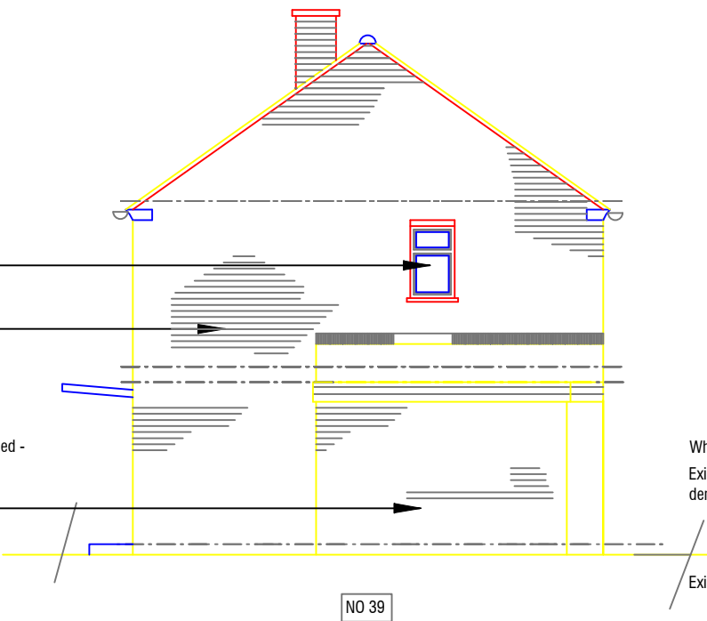
Gable Elevation - As Existing
