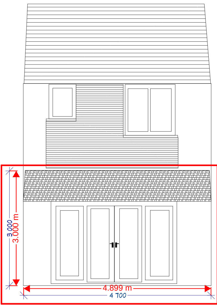
Proposed Rear (SSW) Elevation 1:50
