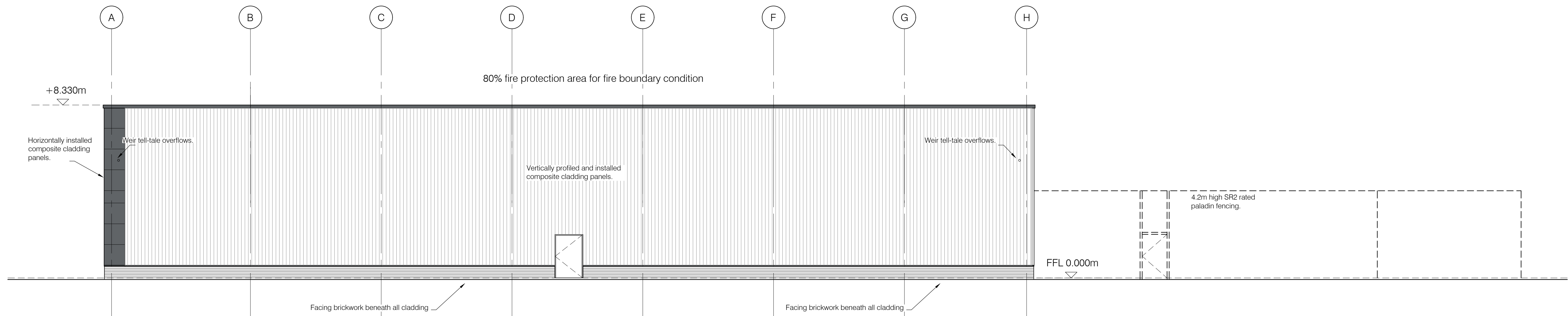
West Elevation
