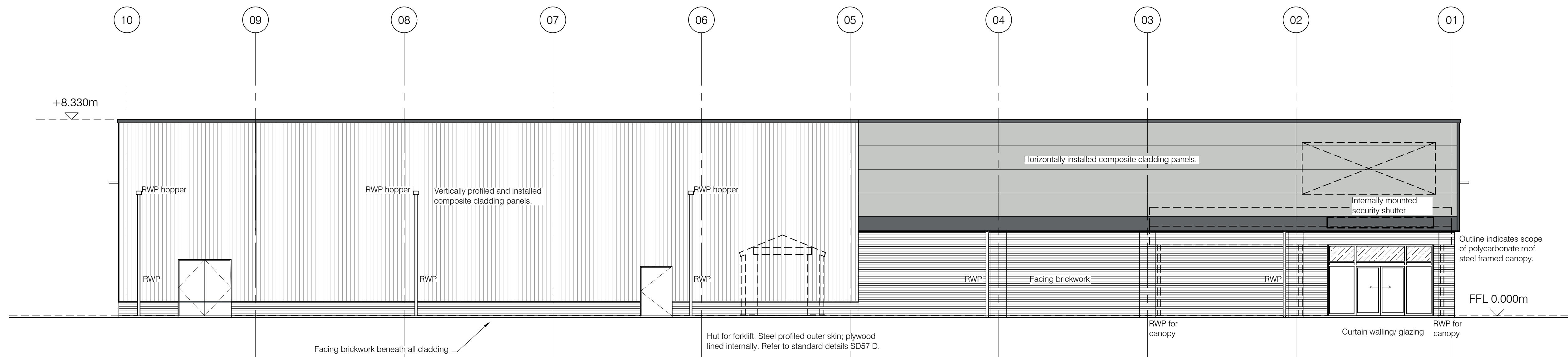
South Elevation
