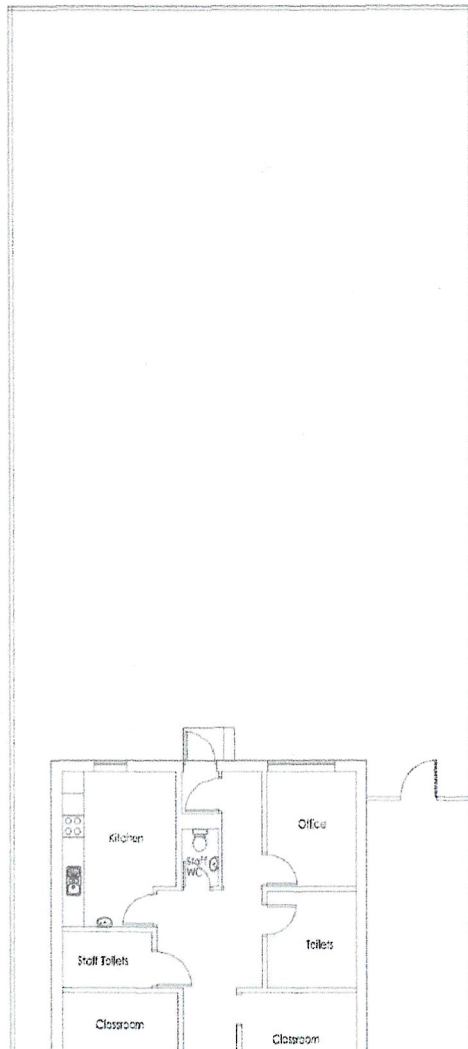
EXISTING GROUND FLOOR PLAN 1:50 @ A0
