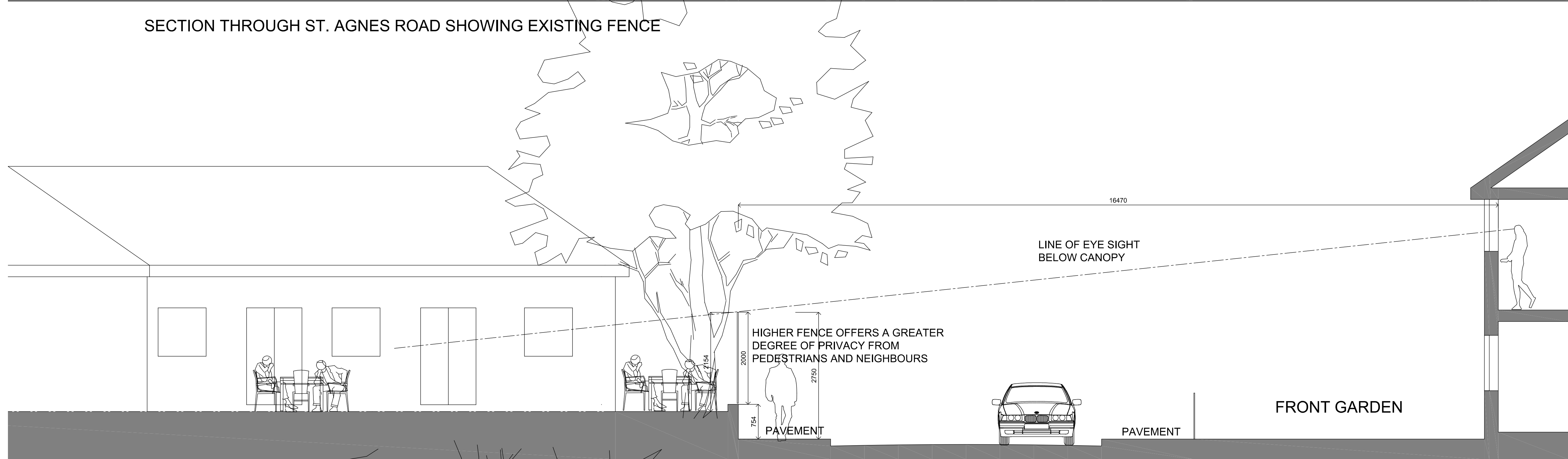
PROPOSED SECTION THROUGH ST. AGNES ROAD SHOWING PROPOSED FENCE
