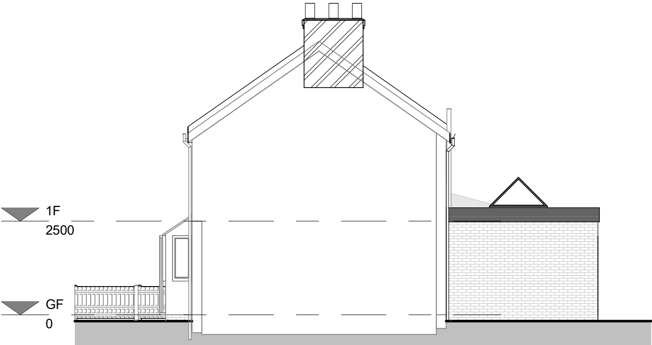
EXISTING SIDE ELEVATION I
