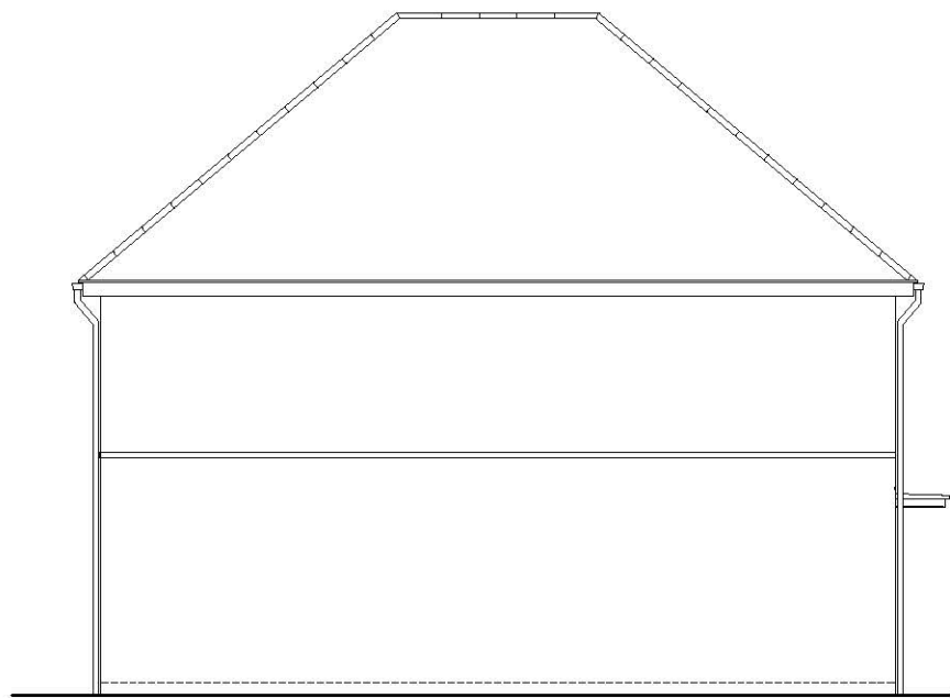
SIDE (LEFT) ELEVATION - AS DETACHED EMA43 (4B5P)
