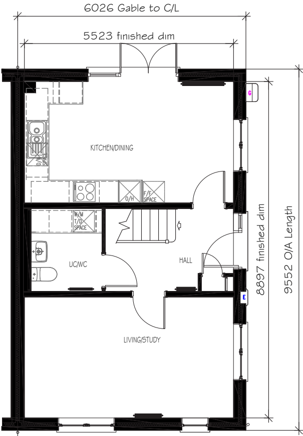
GROUND FLOOR PLAN (END/SEM) EMT31 (3B5P)
