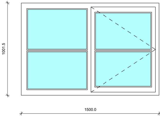
WINDOW TYPE 2
