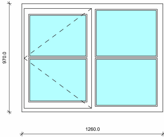
WINDOW TYPE 4
