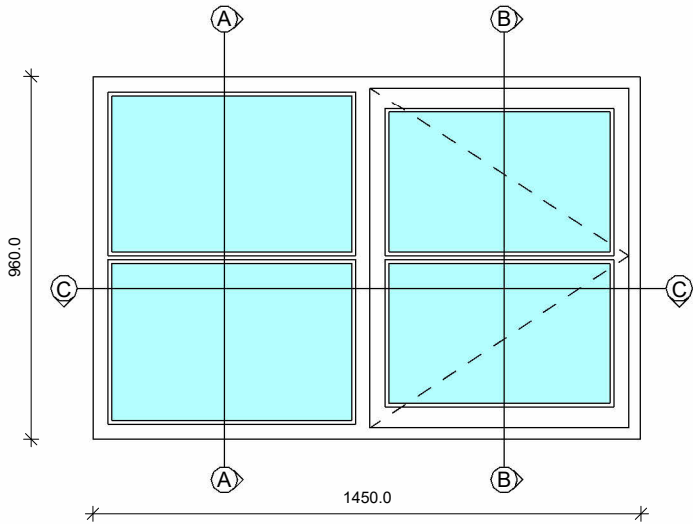
WINDOW TYPE 1
