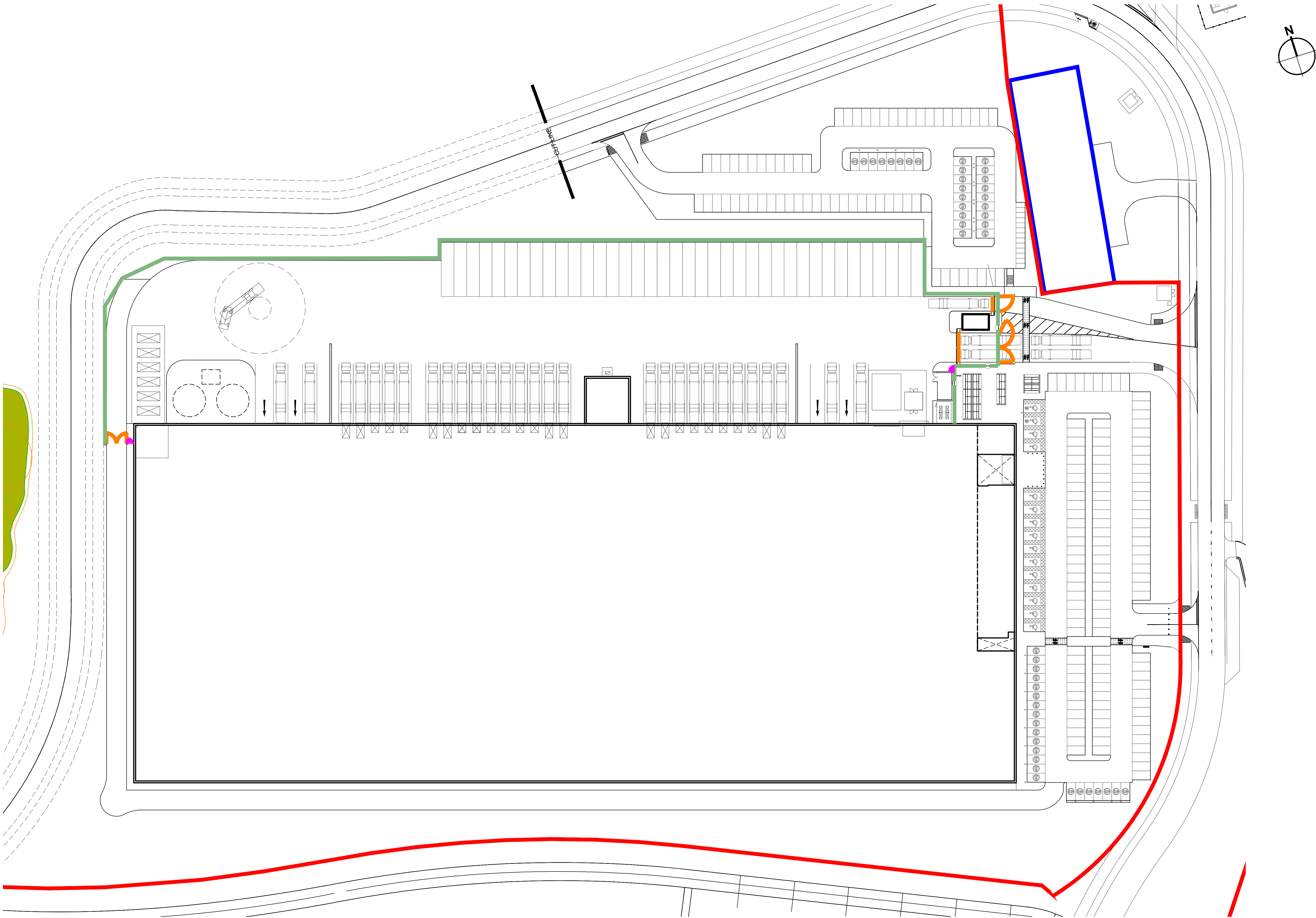
Fencing Plan Scale 1:500
