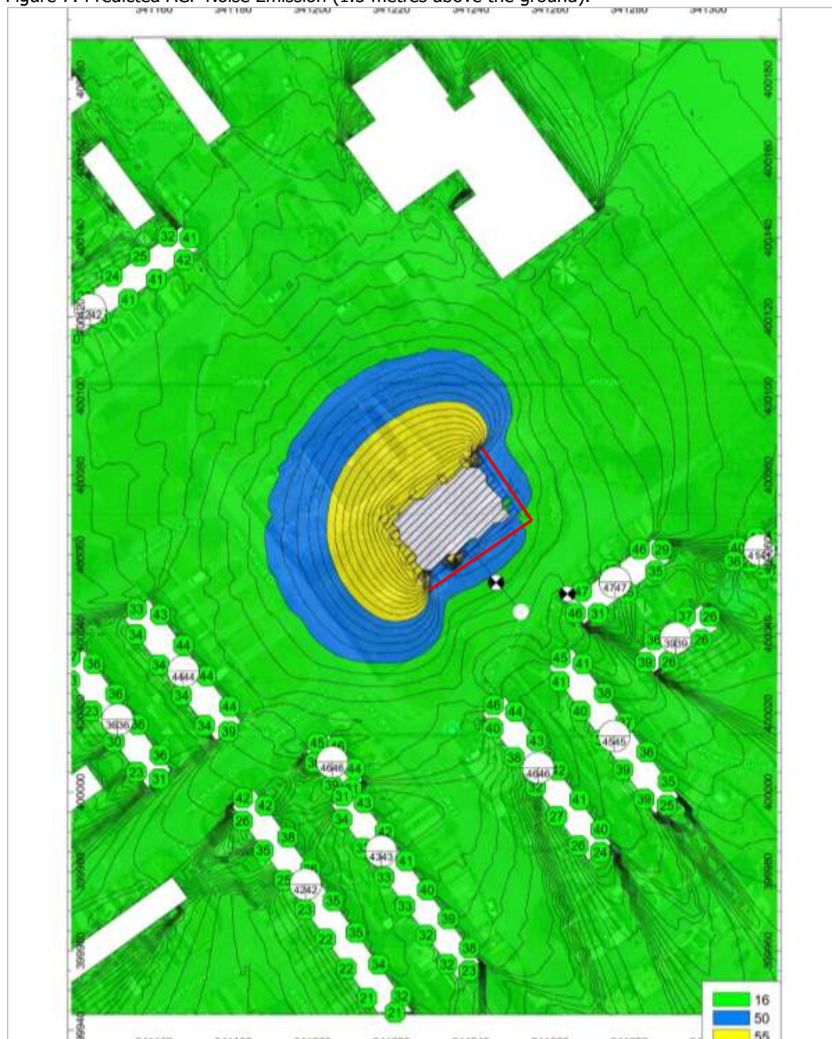
Figure 7: Predicted AGP Noise Emission (1.5 metres above the ground).
