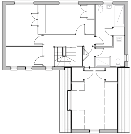
Existing 1st Floor Plan 1:200
