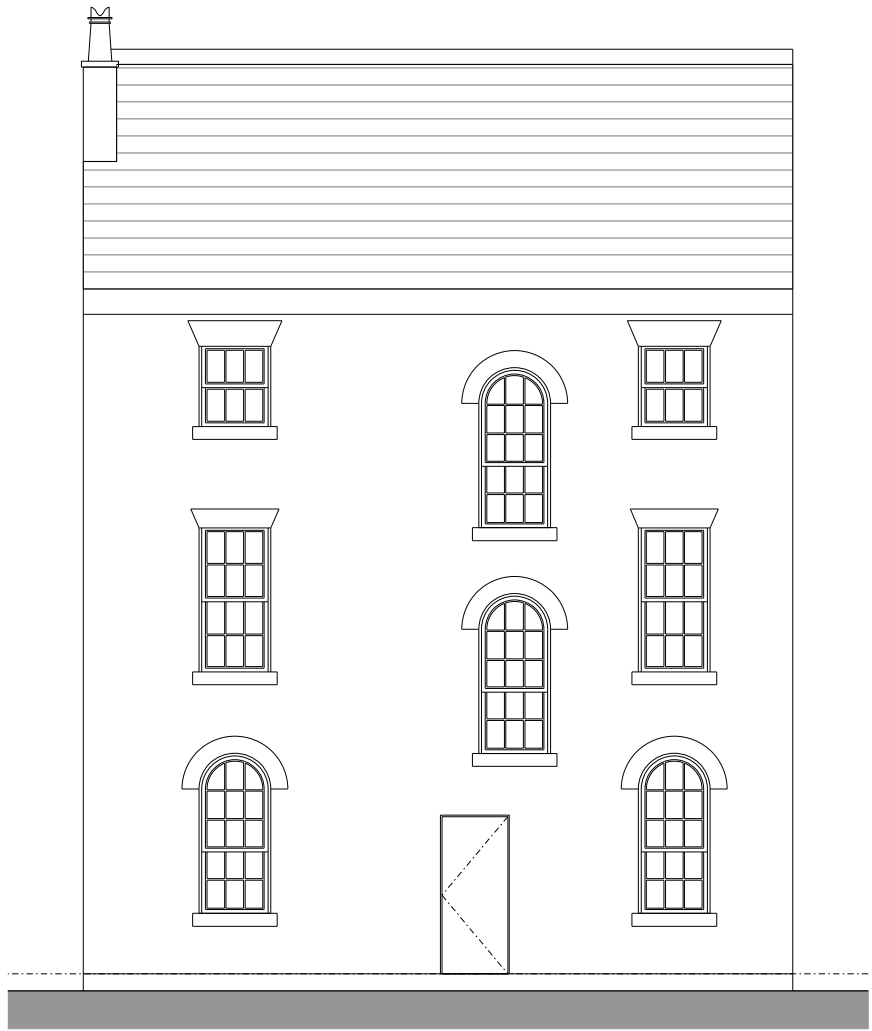
REAR ELEVATION
