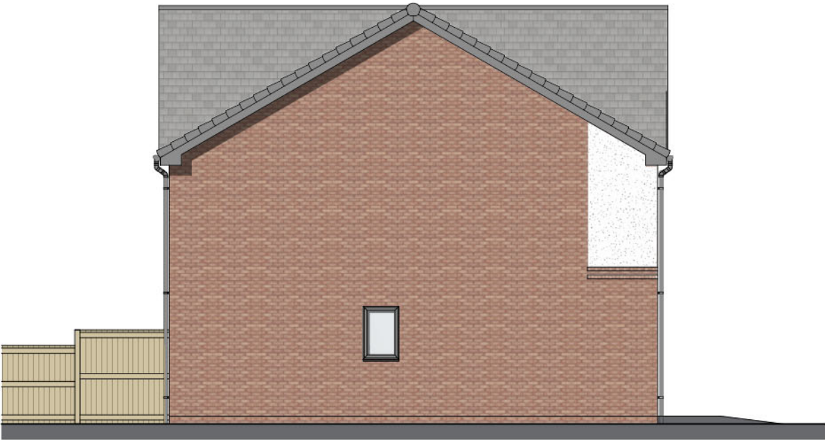
TYPE F 3B4P 86 (AS) SIDE ELEVATION
