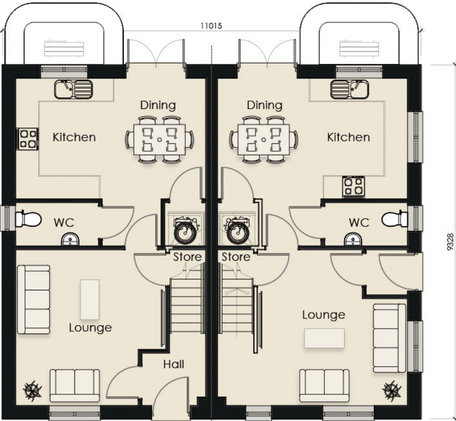
TYPE F - L1F 3B4P 86 (AS) GROUND FLOOR PLAN - Semi-Detached
