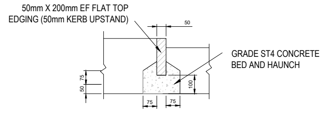
CONCRETE EDGING KERB: 50mm KERB UPSTAND
