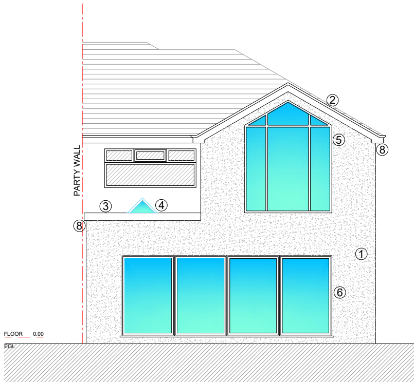
REAR ELEVATION
