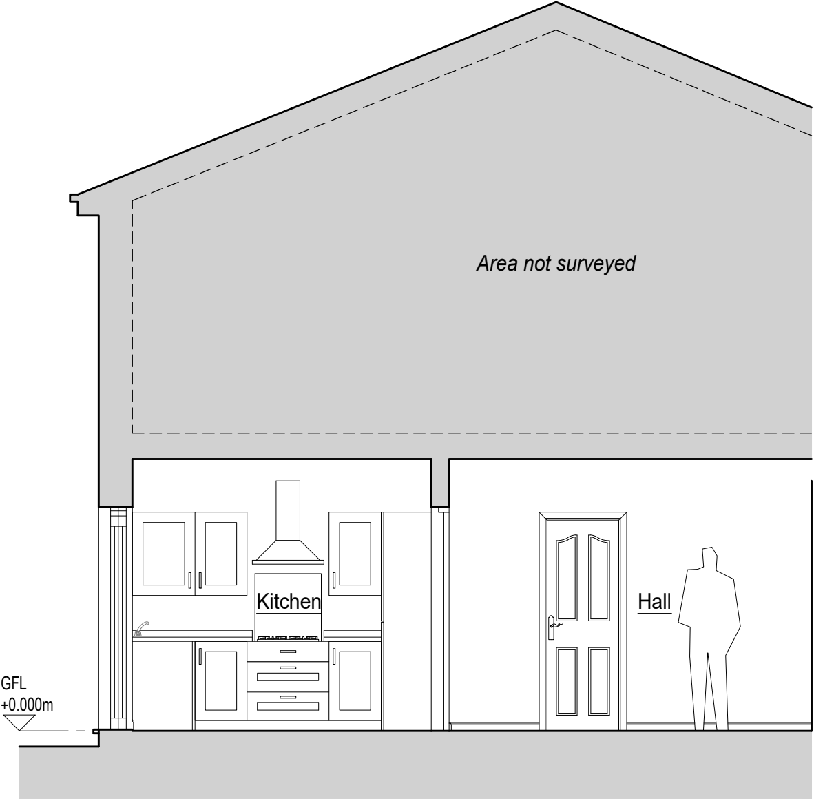
Section A-A as Existing
