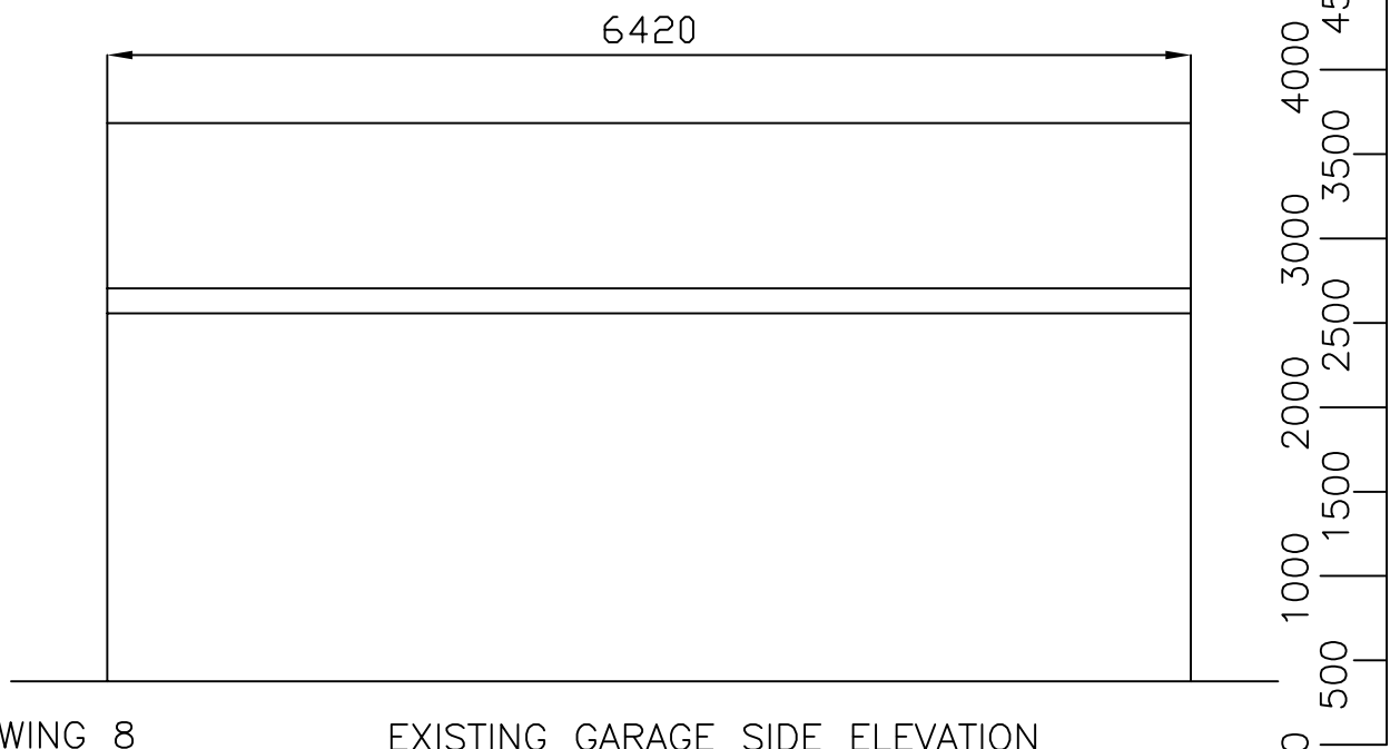
EXISTING GARAGE SIDE ELEVATION
