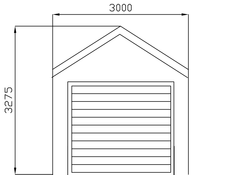
EXISTING GARAGE FRONT ELEVATION
