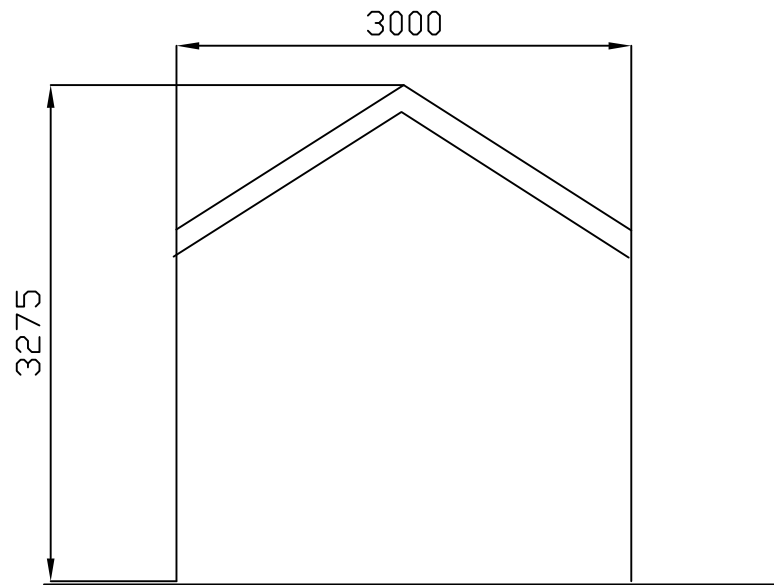
EXISTING GARAGE REAR ELEVATION
