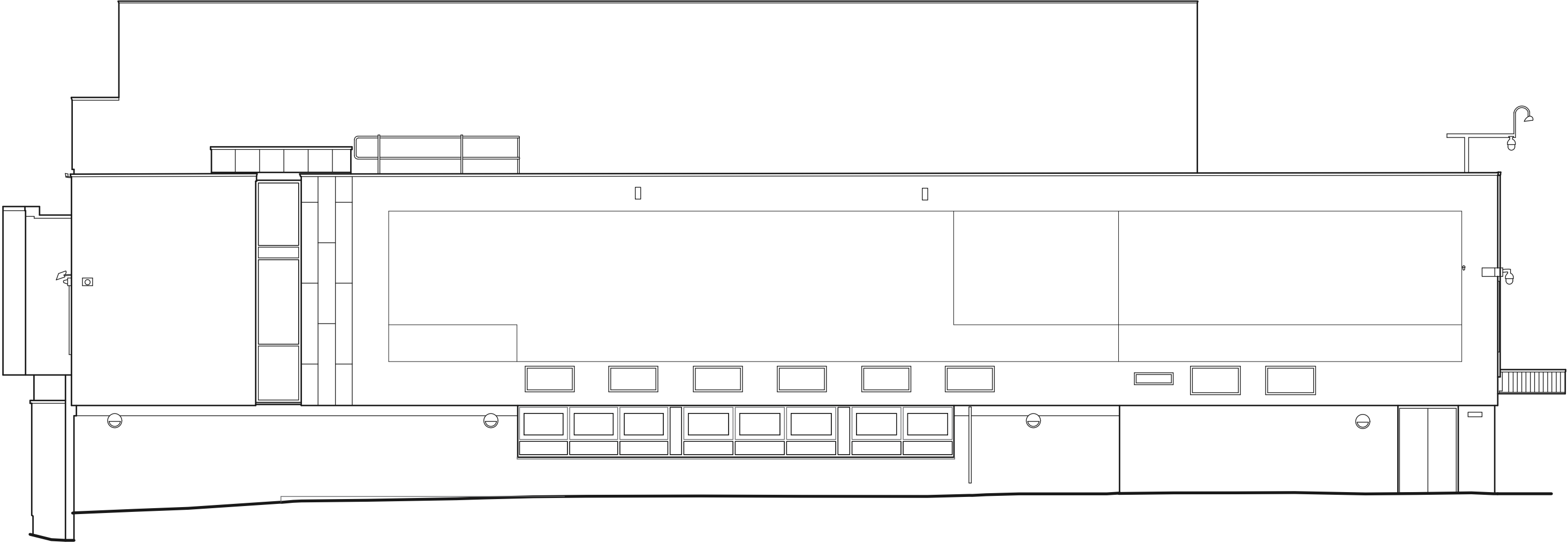
South Elevation
