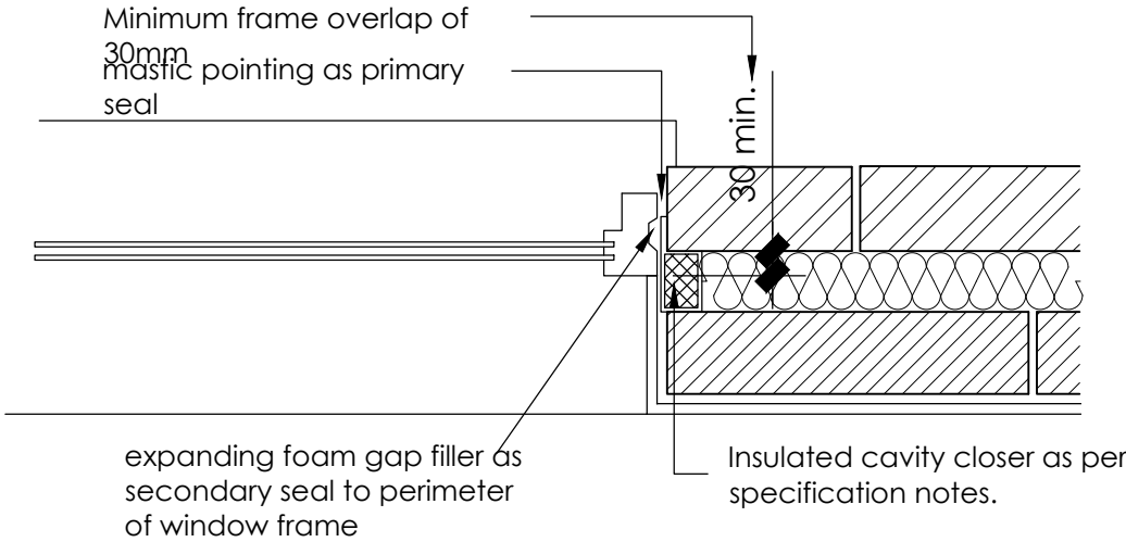
Proposed Window Jamb Detail (Scale - NTS) (Detail to be constructed in accordance with 'Acredited Construction Details' published by BRE)
