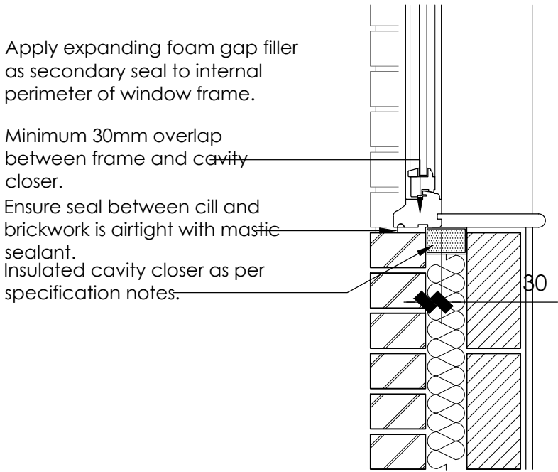
Proposed Window Head and Sill - Brickwork
