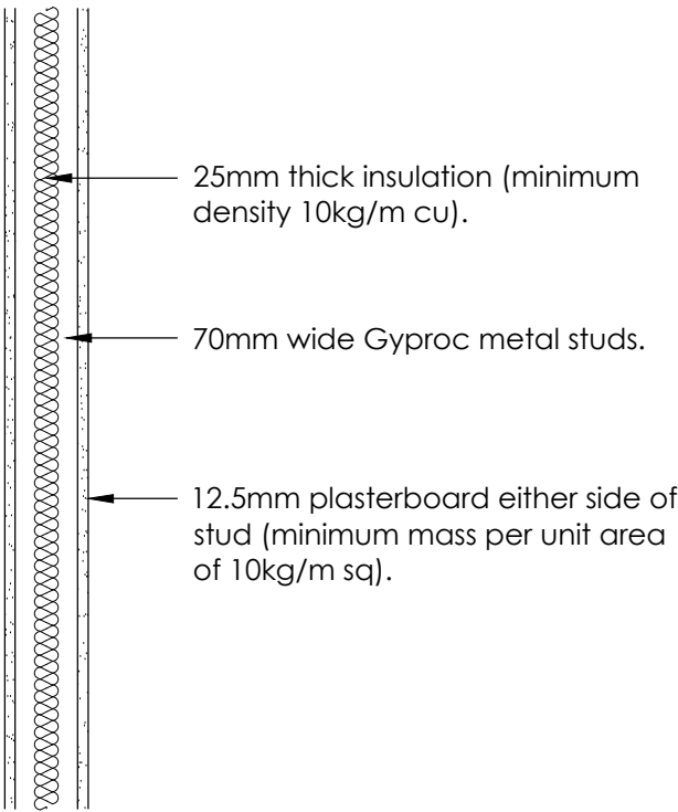
Proposed Metal Stud Partition (Achieves 30min Fire Resistance)
