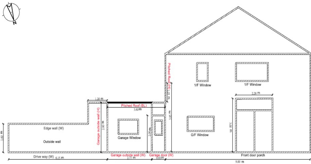
EXISTING FRONT SIDE ELEVATION
